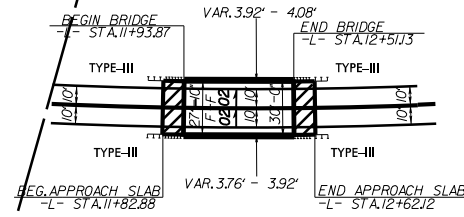
SKETCH SHOWING BRIDGE/PAVEMENT RELATIONSHIP
