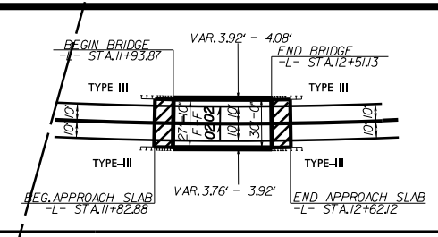
SKETCH SHOWING BRIDGE/PAVEMENT RELATIONSHIP
